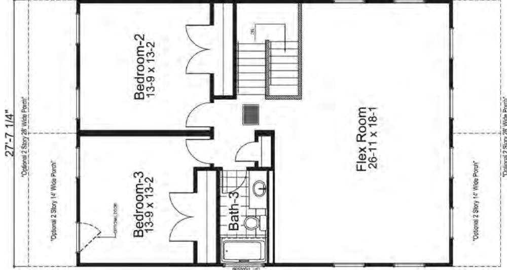
SECOND LEVEL FLOOR PLAN
