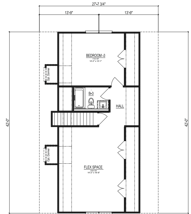
SUGGESTED UPPER LEVEL LAYOUT IF FINISHED
