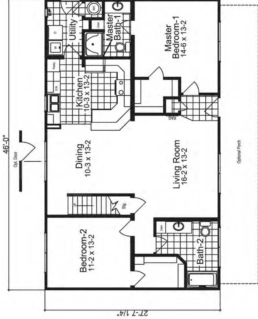
FIRST LEVEL FLOOR PLAN
